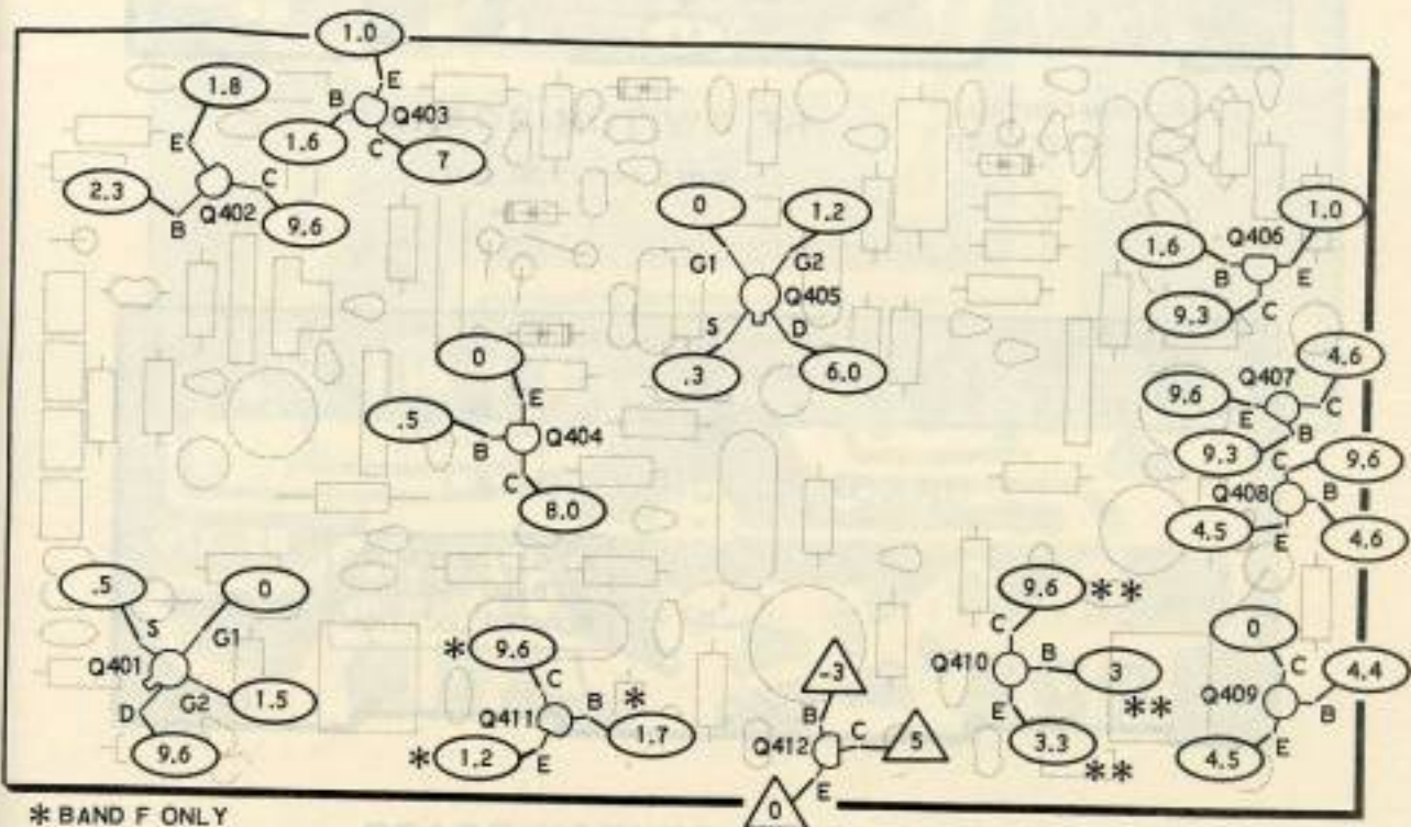
RECEIVER CIRCUIT BOARD (VIEWED FROM COMPONENT SIDE)
